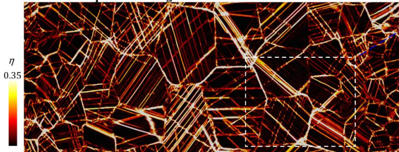
Dislocation slip and twinning
